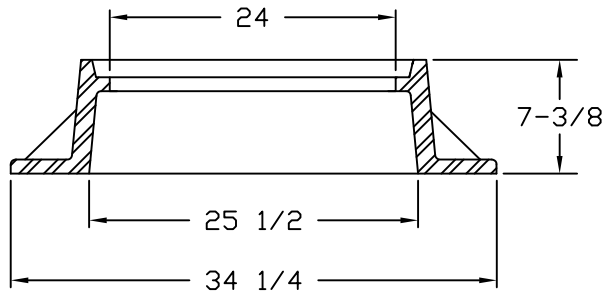
RING - SECTION
