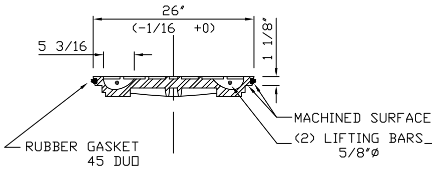
COVER - SECTION
