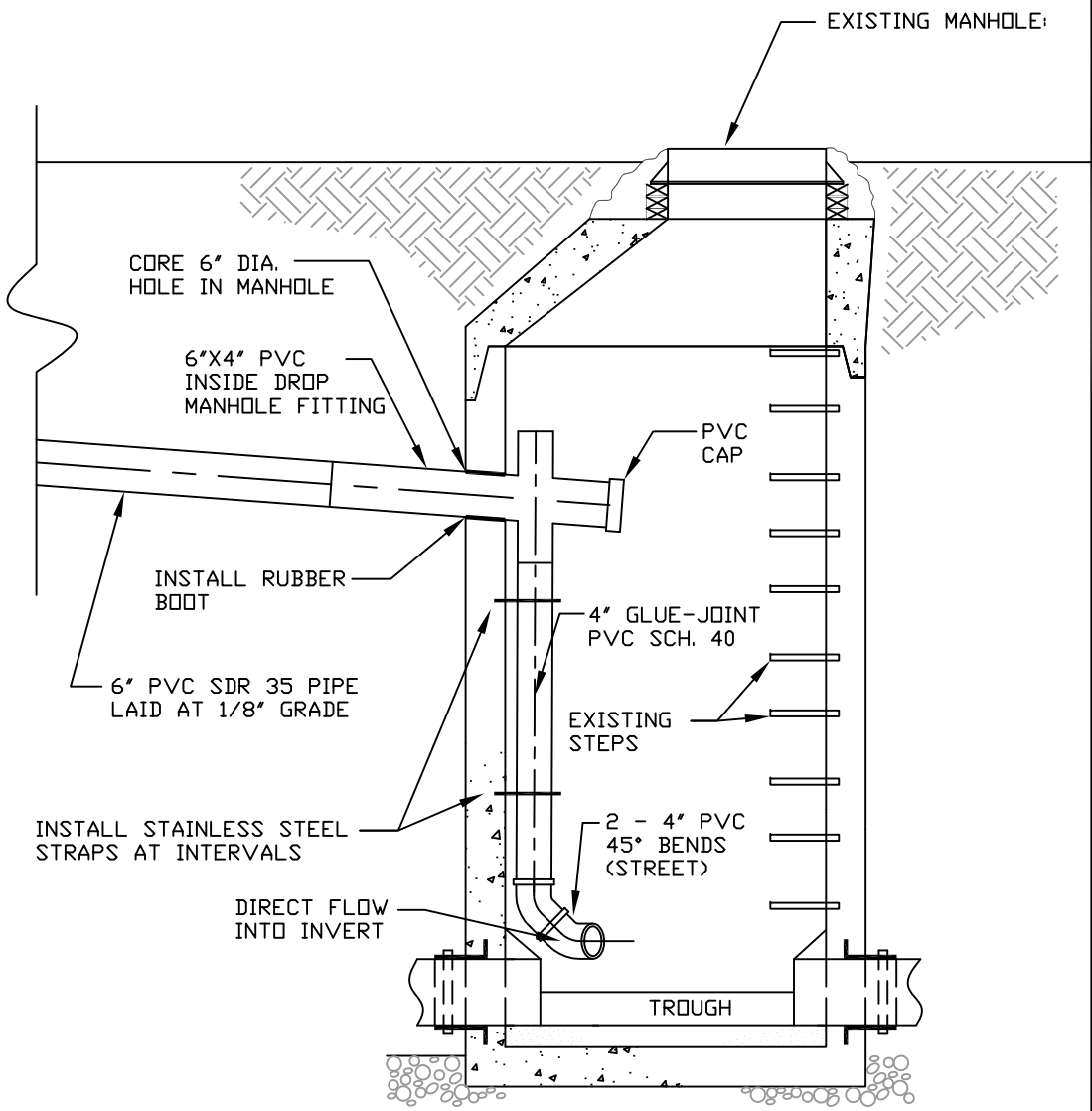
SECTION DETAIL NOT TO SCALE
